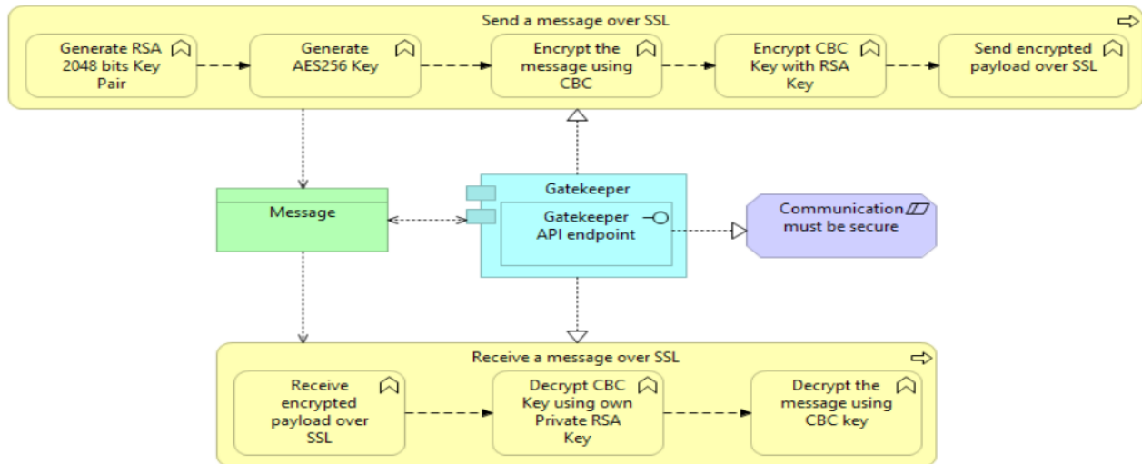
Figure 2 – Enhanced Gatekeeper implementation
